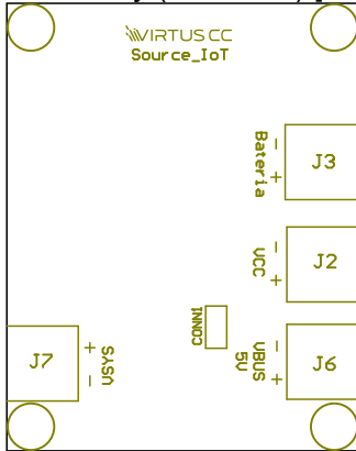
Bottom Overlay (Scale 1:1) [Bottom]
