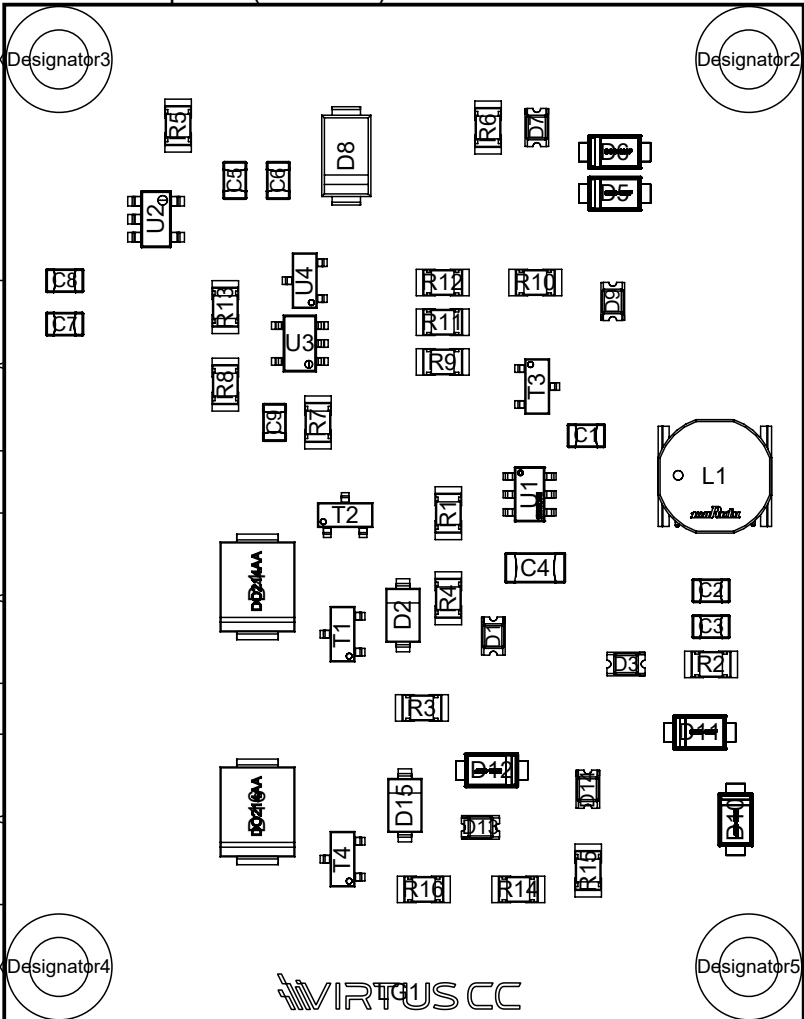
View from Top side (Scale 5:2)
