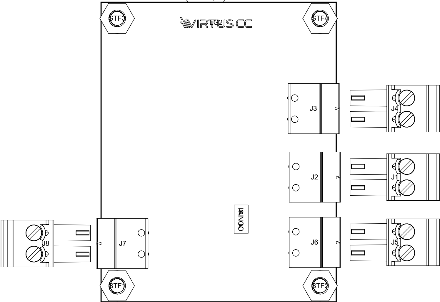
View from Bottom side (Scale 5:2)
