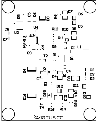
Top Overlay (Scale 1:1) [Top]
