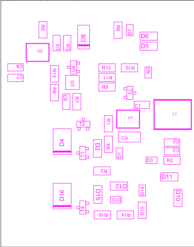
Top Assembly (Scale 5:2)
