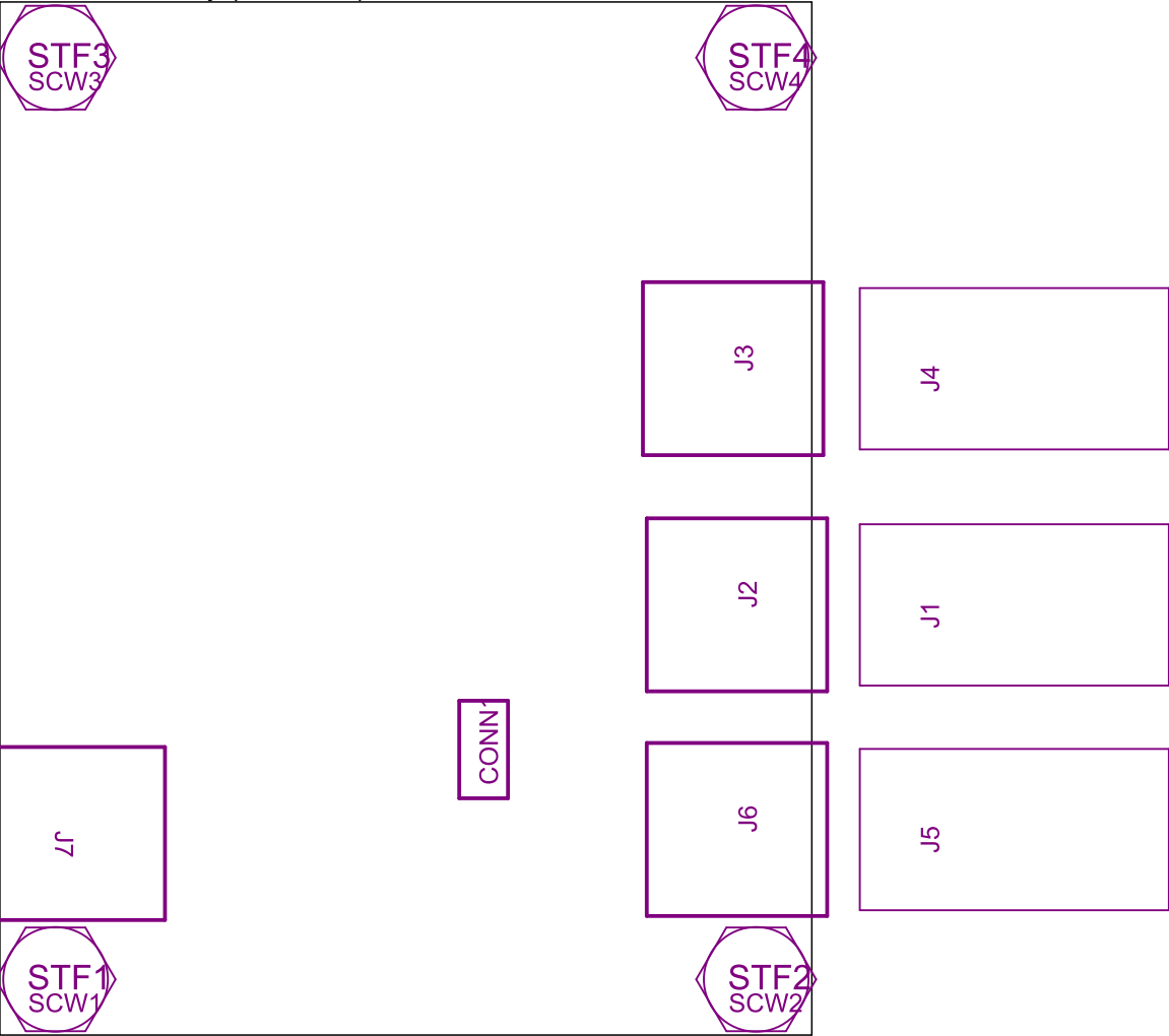
Bottom Assembly (Scale 5:2)
